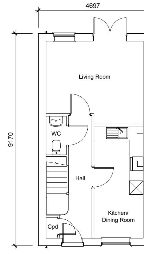
Type 27 Ground Floor Plan 2-Bedroom House 71.4sqm / 769sqft GIA [to finishes]
