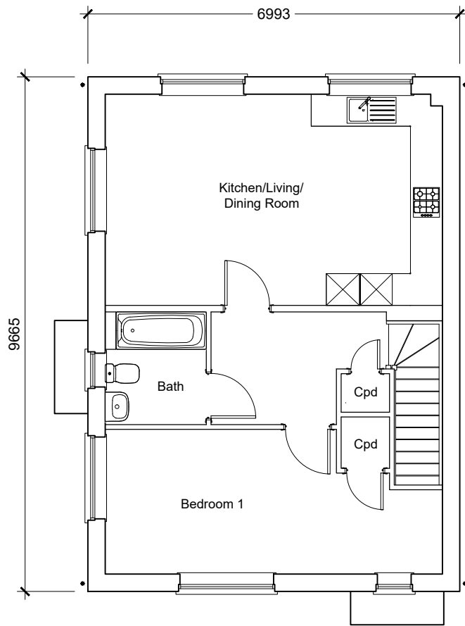
First Floor Plan 1-Bedroom 2-Person Flat 61.9sqm / 666.5sqft GIA [to finishes]
