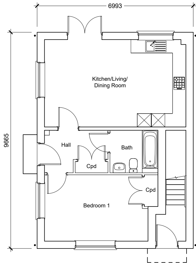
Type 1 Ground Floor Plan 1-Bedroom 2-Person Flat 50.0sqm / 533sqft GIA [to finishes]
