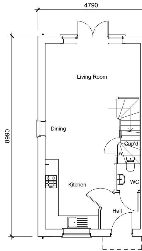
Type 3 Ground Floor Plan 2-Bedroom House 71.5sqm / 770sqft GIA [to finishes]
