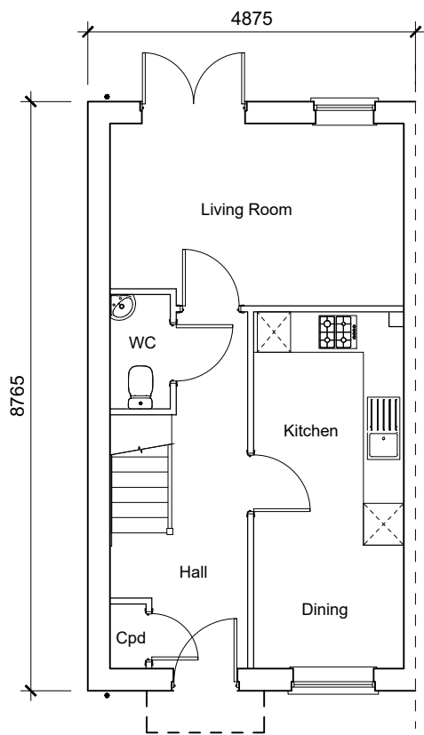
Type 2 Ground Floor Plan 2-Bedroom 3-Person House 70.9sqm / 763sqft GIA [to finishes]
