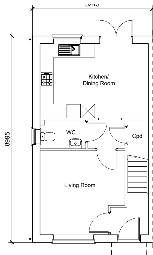
Type 5 Ground Floor Plan 2-Bedroom House 79.06sqm / 851sqft GIA [to finishes]
