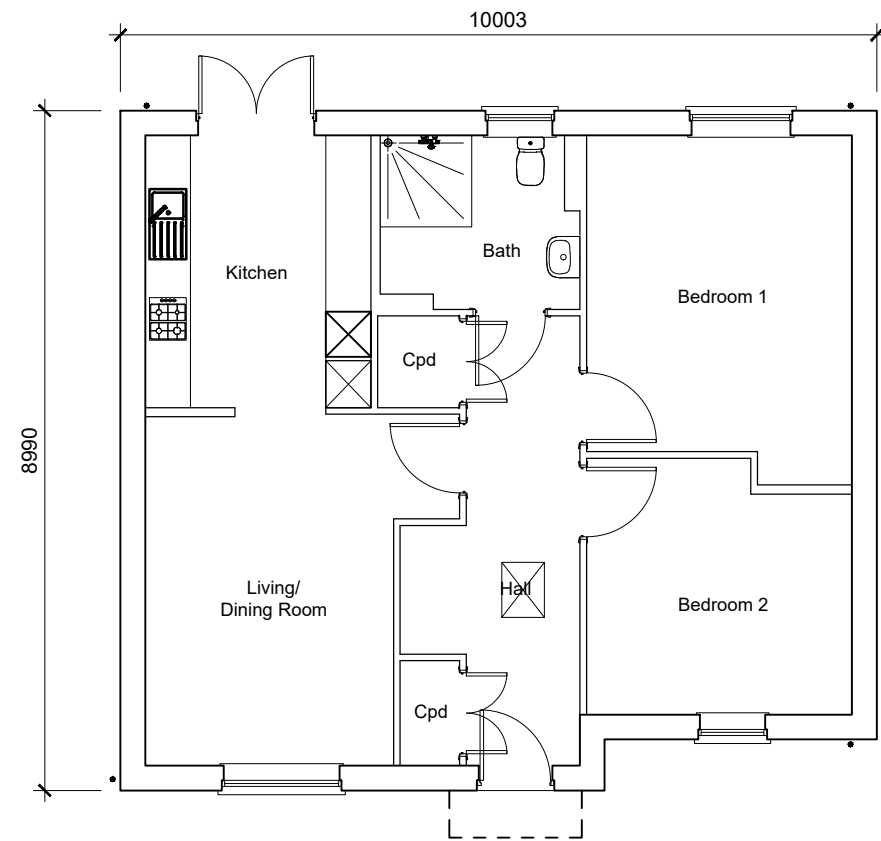
Type 4 Ground Floor Plan 2-Bedroom 3-Person House M(4)3 75.4sqm / 812sqft GIA [to finishes]
