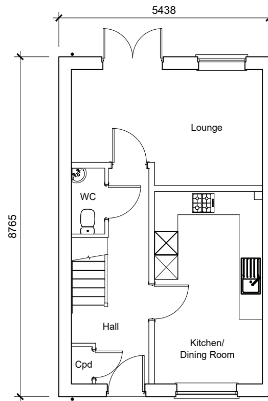
Type 6 Ground Floor Plan 2-Bedroom 4-Person House 80.1sqm / 862sqft GIA [to finishes]
