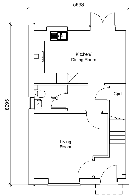
Type 7 Ground Floor Plan 3-Bedroom House 86.5sqm / 932sqft GIA (to finishes)
