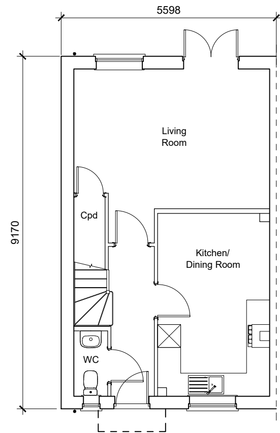
Type 8 Ground Floor Plan 3-Bedroom House 86.7sqm / 934sqft GIA (to finishes)
