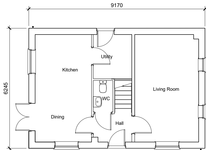
Type 10 Ground Floor Plan 3-Bedroom House 95.2sqm / 1025sqft GIA (to finishes)
