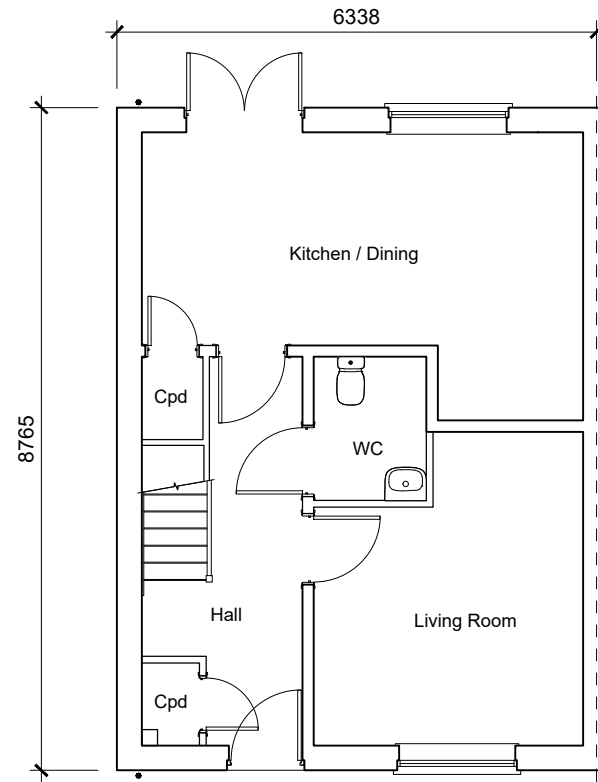
Type 9 Ground Floor Plan 3-Bedroom 5-Person House 94.6sqm / 1019sqft GIA (to finishes)
