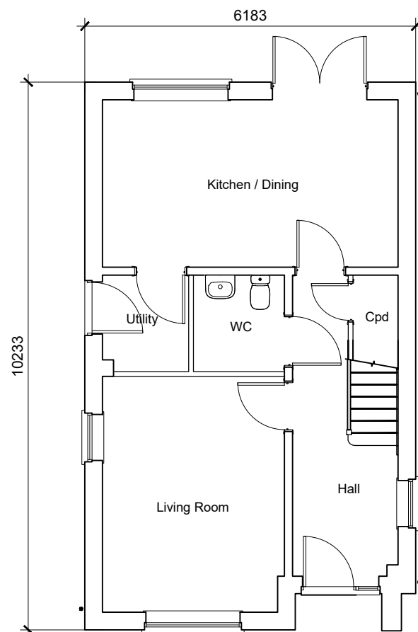
Type 12 Ground Floor Plan
