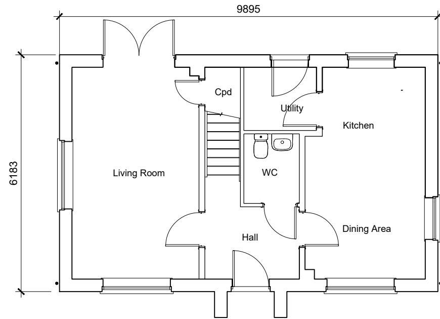
Type 11 Ground Floor Plan
