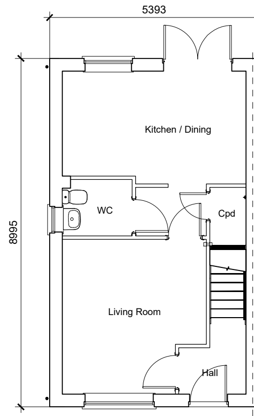
Type 13 Ground Floor Plan 3-Bedroom House 104.4sqm / 1124sqft GIA (to finishes)
