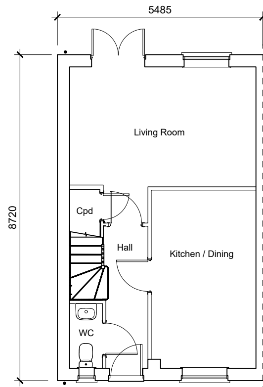
Type 14 Ground Floor Plan 4-Bedroom House 102.94sqm / 1108sqft GIA [to finishes]
