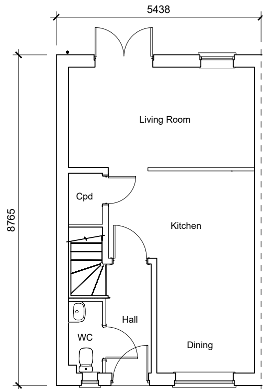
Type 15 Ground Floor Plan 3-Bedroom 5-Person House 103.8sqm / 1117.28sqft GIA [to finishes]
