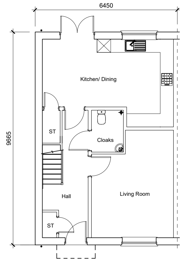
Type 17 Ground Floor Plan 4-Bedroom 5-Person House 107.17sqm / 1153.61sqft GIA [to finishes]
