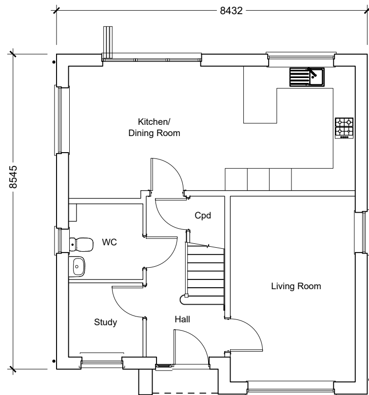
Type 22 Ground Floor Plan 4-Bedroom House 127.3sqm / 1370.24sqft GIA [to finishes]
