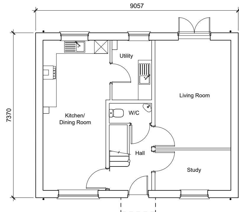
Type 24 Ground Floor Plan 5-Bedroom House 140.55sqm / 1512.83sqft GIA (to finishes)
