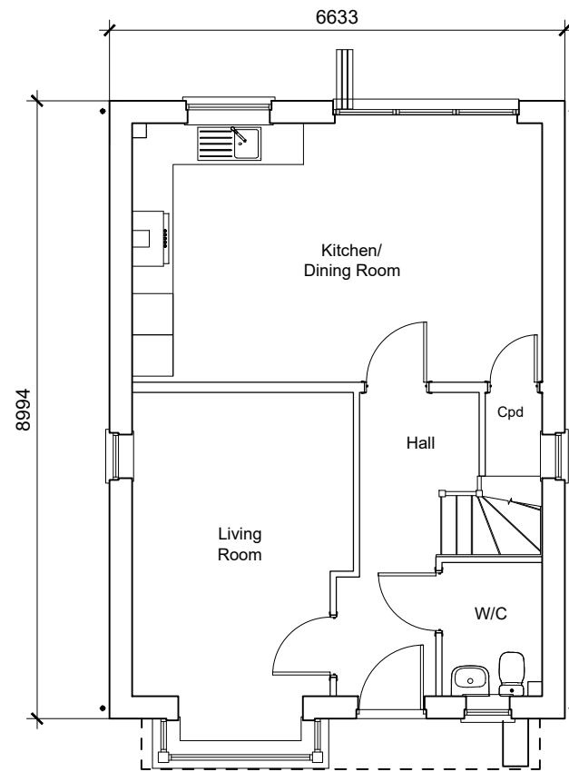
Type 23 Ground Floor Plan 4-Bedroom House 135.56sqm / 1457sqft GIA (to finishes)
