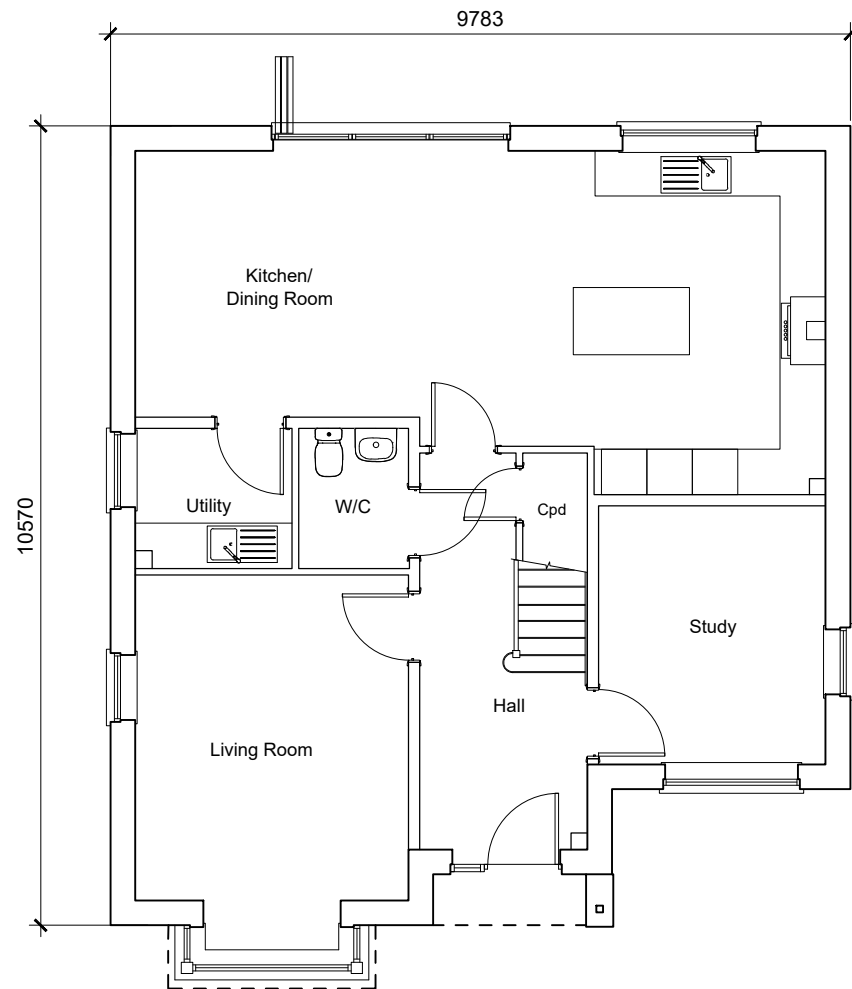
Type 25 Ground Floor Plan 5-Bedroom House 167.75sqm / 1805.64sqft GIA [to finishes]
