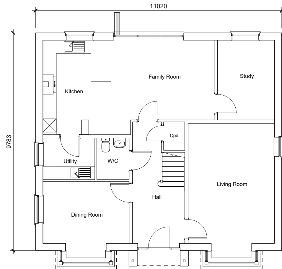
Type 26 Ground Floor Plan 5-Bedroom House 191.66sqm / 2063.05sqft GIA [to finishes]
