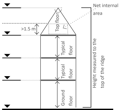
Illustrative Diagrams: Pitched roof design options
