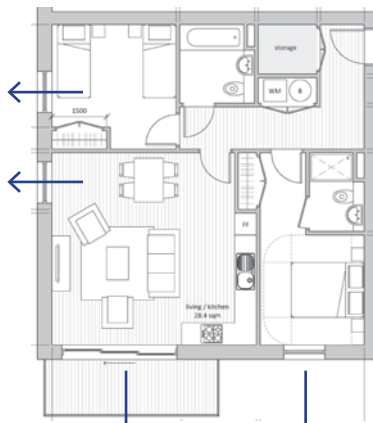
Illustrative - 2B4P dual aspect dwelling
