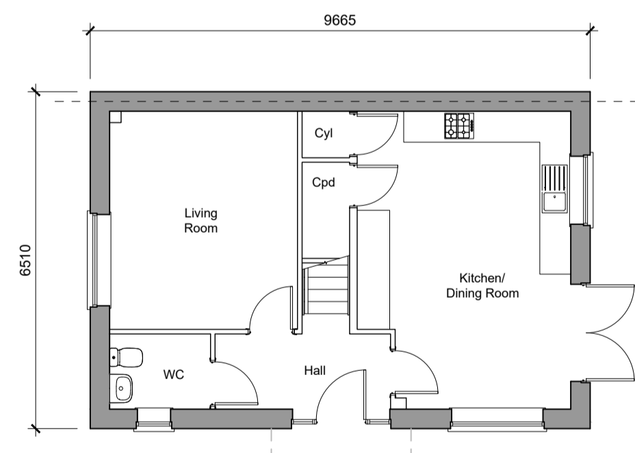
Ground Floor Plan 3-Bedroom House 332 202ppm / 1105sqft GFA (as framed) Plots - 58, 90, 180, 197 Handed - 174
