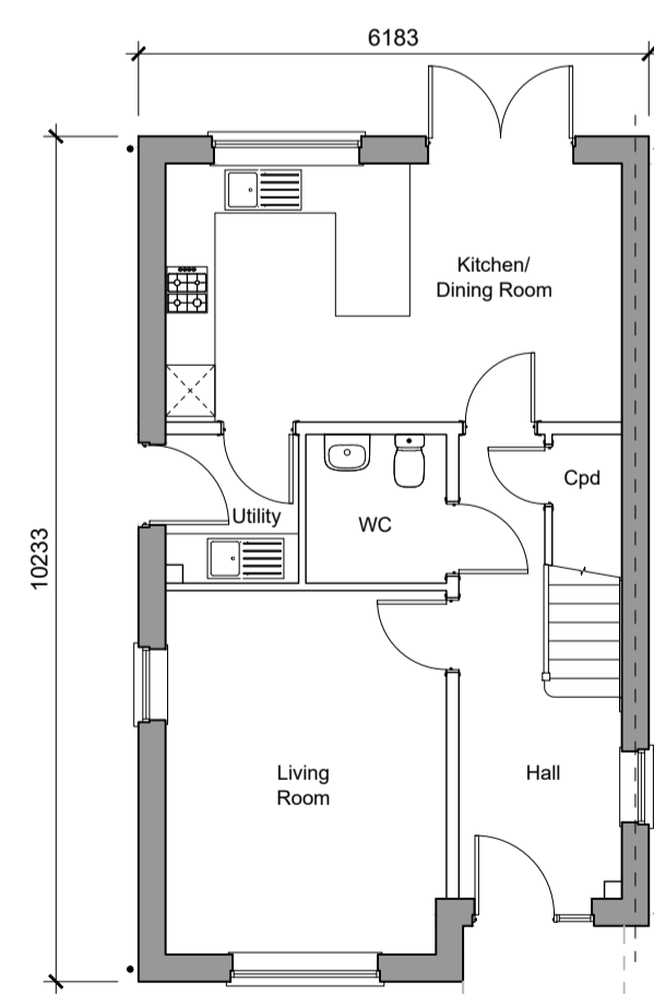
Ground Floor Plan 3-Bedroom House 102.86sqm/1107sqft (GIA, to be used) Plots - 26, 119, 140 Handed - 9, 25
