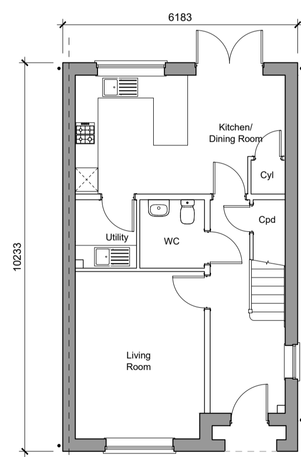
Ground Floor Plan 3-Bedroom House 102.86sqm / 1107sqft GIA (to include) Plots - 113 Handed - 114
