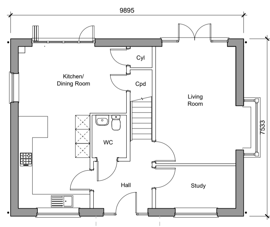
Ground Floor Plan 4-Bedroom House 127 (Open) / 1366sqR GIA (to include) Plot - 31
