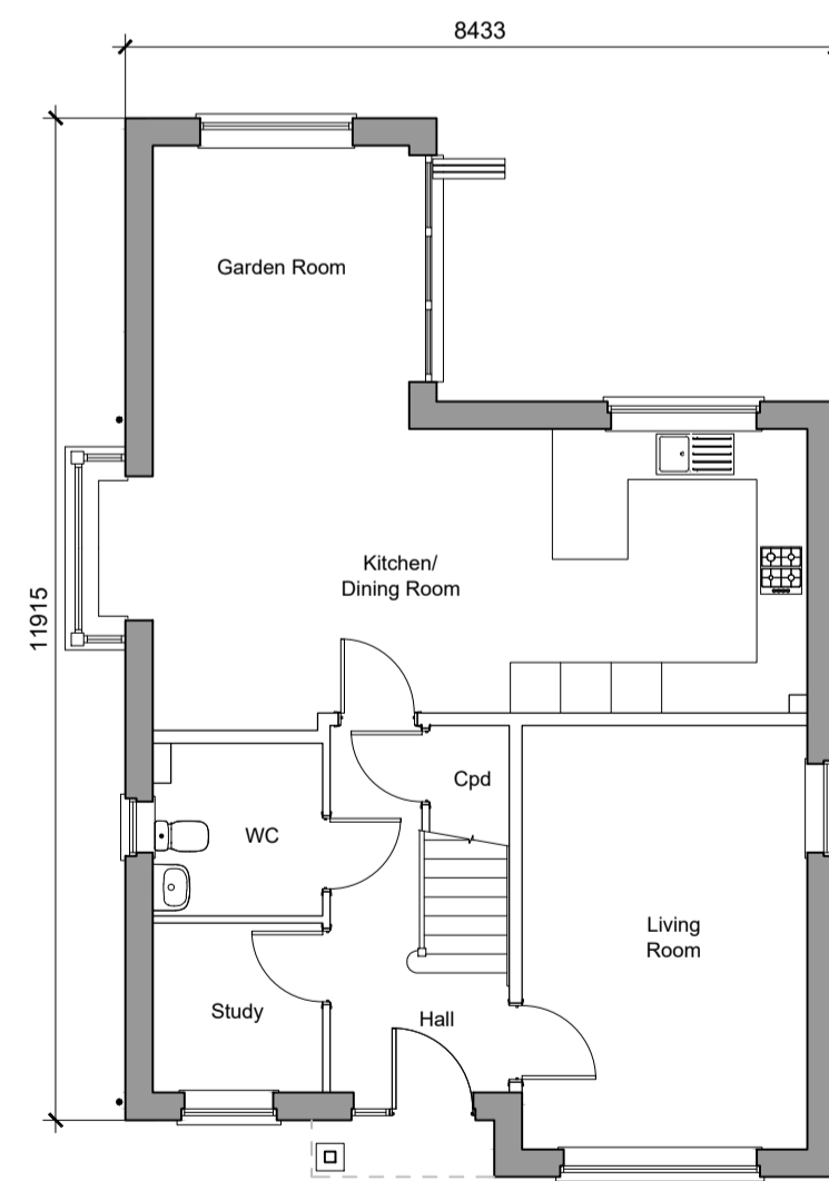
Ground Floor Plan 4-Bedroom House 138.41sqm / 1489sqft GIA (to finished) Plots - 45, 141 Handed - 129
