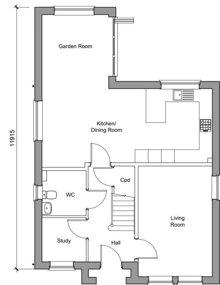
Ground Floor Plan 4-Bedroom House 137.31sqm / 1478sqft GIA (to include) Plot - Handled - 4
