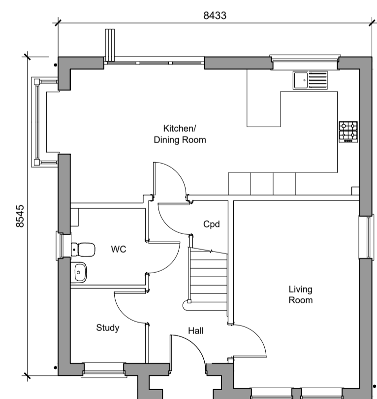
Ground Floor Plan 4-Bedroom House 127 St Leonards Road, Reading, RG2 1BA Plot - Handed - 2
