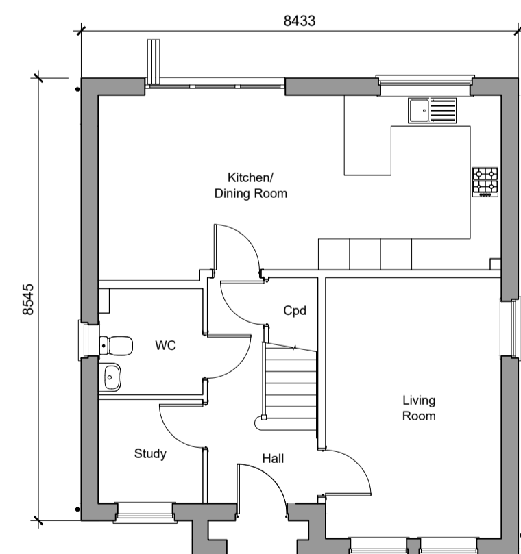
Ground Floor Plan 4-Bedroom House 127.31sqm / 1370sqft GIA Plots - 115 Handed - 3, 109
