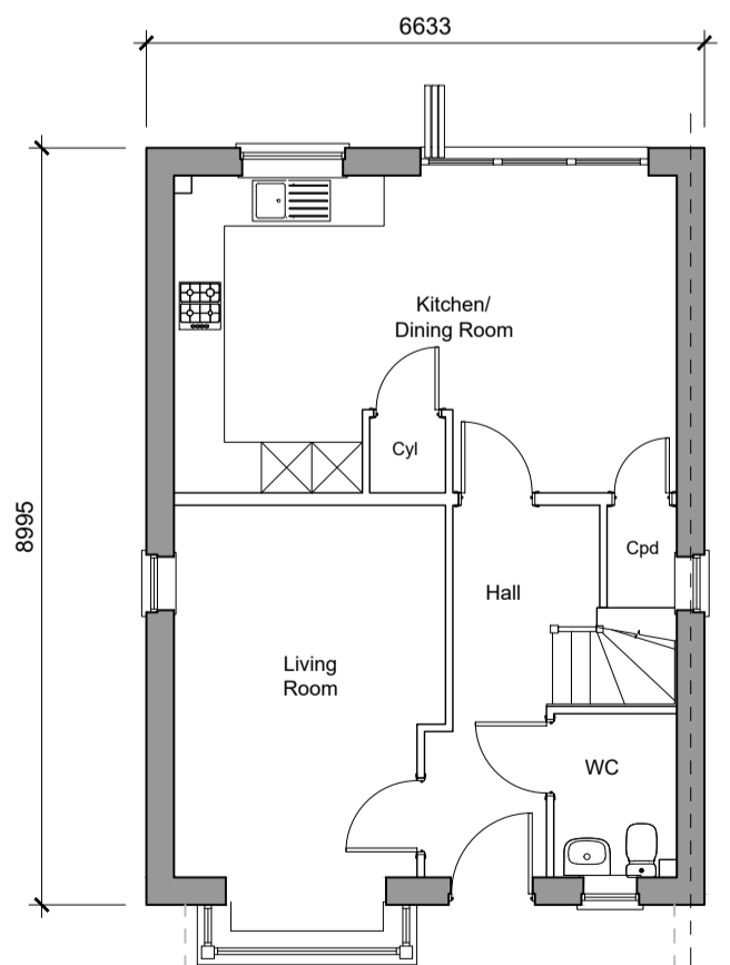
Ground Floor Plan 4-Bedroom House 135.36sqm / 1457.09sqft GFA Plots - 40, 42, 121, 157, 160, 161 Handed - 39, 41, 120, 150, 156
