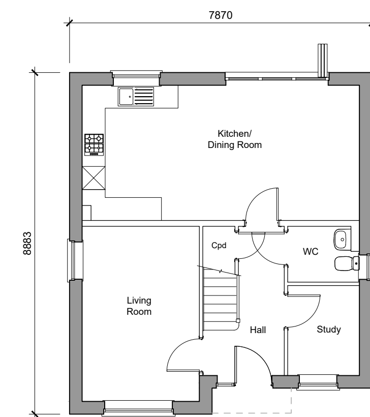
Ground Floor Plan 4-Bedroom House 113 (Approx. 1218sq ft) (in house) Plots 98, 108, 158 Handled - 112, 149, 155
