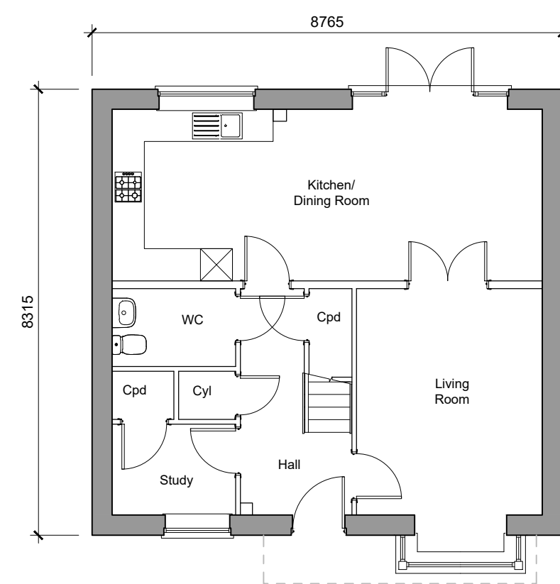
Ground Floor Plan 4-Bedroom House 122.45sqm / 1318sqft GIA (to finished) Plots - 67, 70, 74, 86
