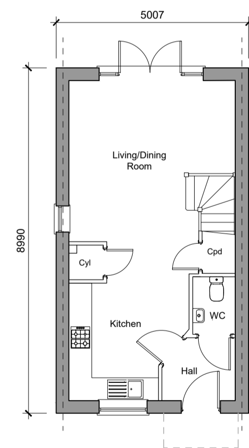
Ground Floor Plan 2-Bedroom 4-Person House 72.18sqm / 776sqft GFA, 19.1sqm Plots - 7, 30, 34, 36, 38, 148 Handed - 6, 29, 33, 35, 37, 146, 147
