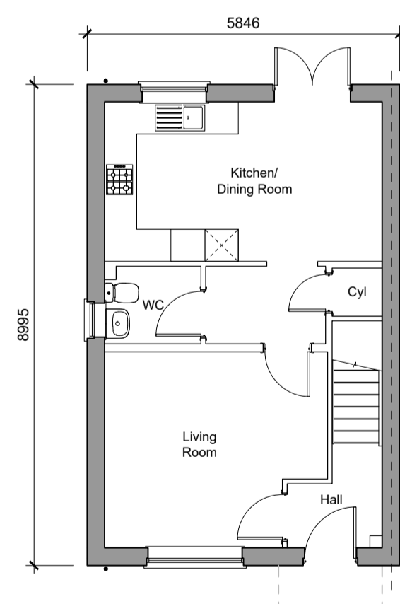
Ground Floor Plan 3-Bedroom House 86.57sqm (1018ft 2 GA, 3p. house) Plots - 46, 97, 100, 111, 143, 152, 154 Handed - 47, 96, 101, 110, 142, 151, 153
