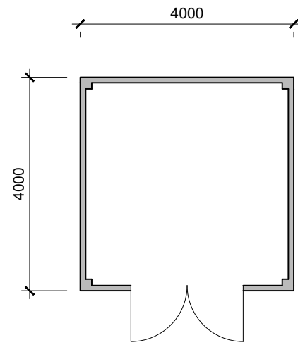
Sub Station Floor Plan
