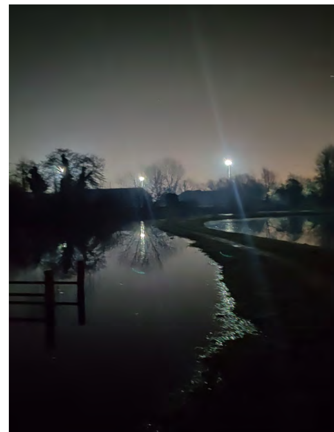
Light pollution over the Fobney Island Nature Reserve from the Thames Water treatment plant
