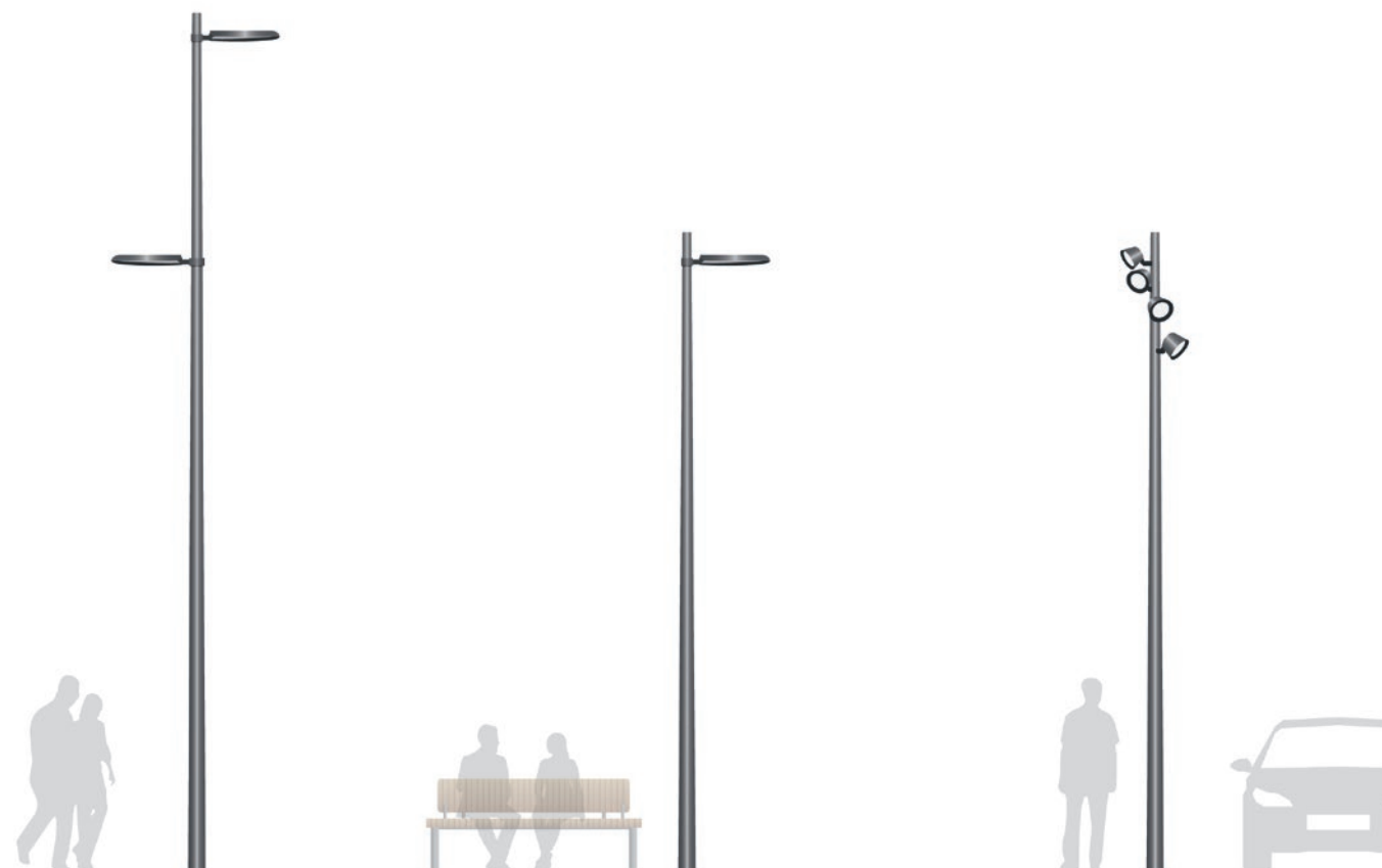
Typical Lighting Column 1 8m tapered or cylindrical column 1 or 2 single pole luminaires Street lighting optics
